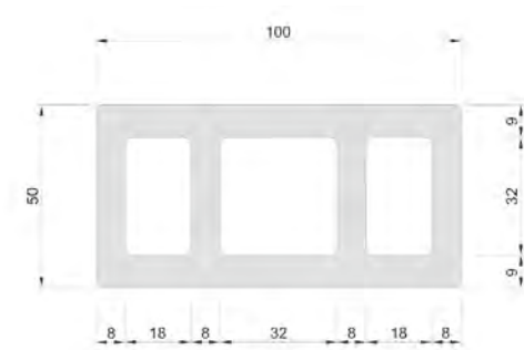
Barro 50x100 mm max. length = 1.700 mm
