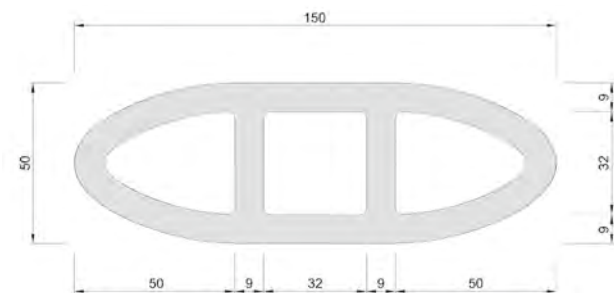
Barro Ellipse 50x150 mm max. length = 1.700 mm
