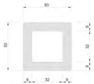
Barro 50x50 mm max. length = 1.700 mm
