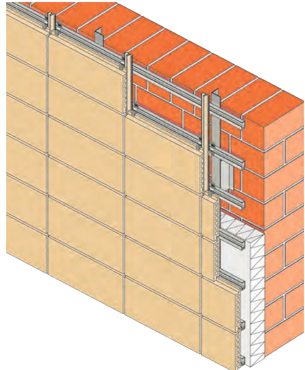
Figure 2 – Horizontal substructure
